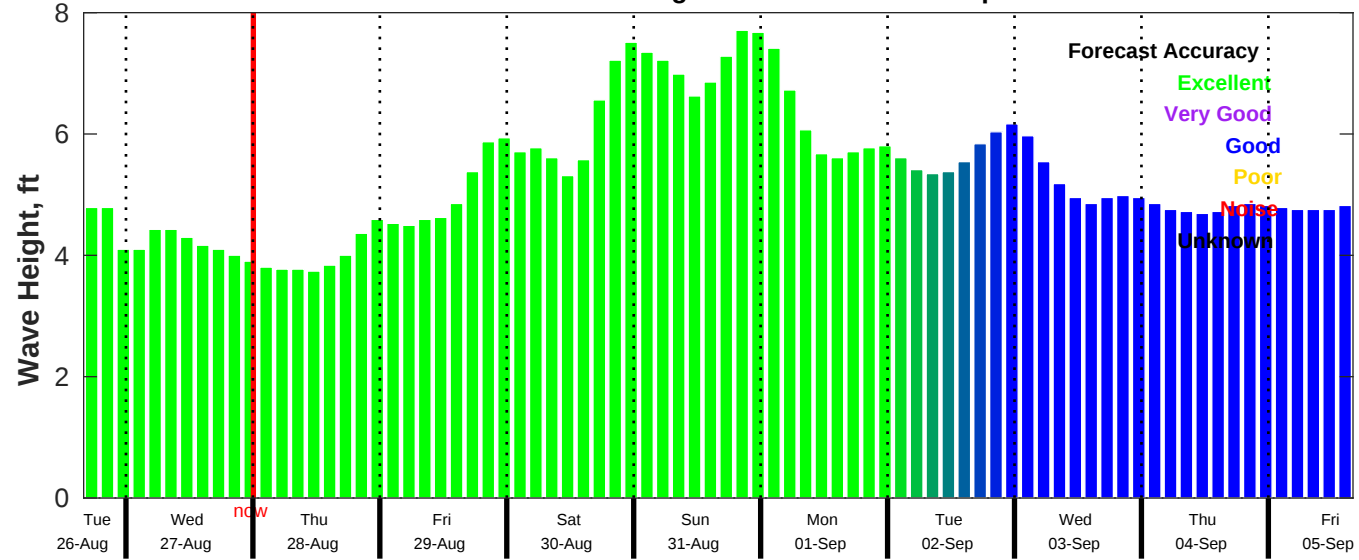
CMEMS Wave Forecast for NDBC 46028 from 26-Aug-2025 16:00:00 to 05-Sep-2025 16:00:00
