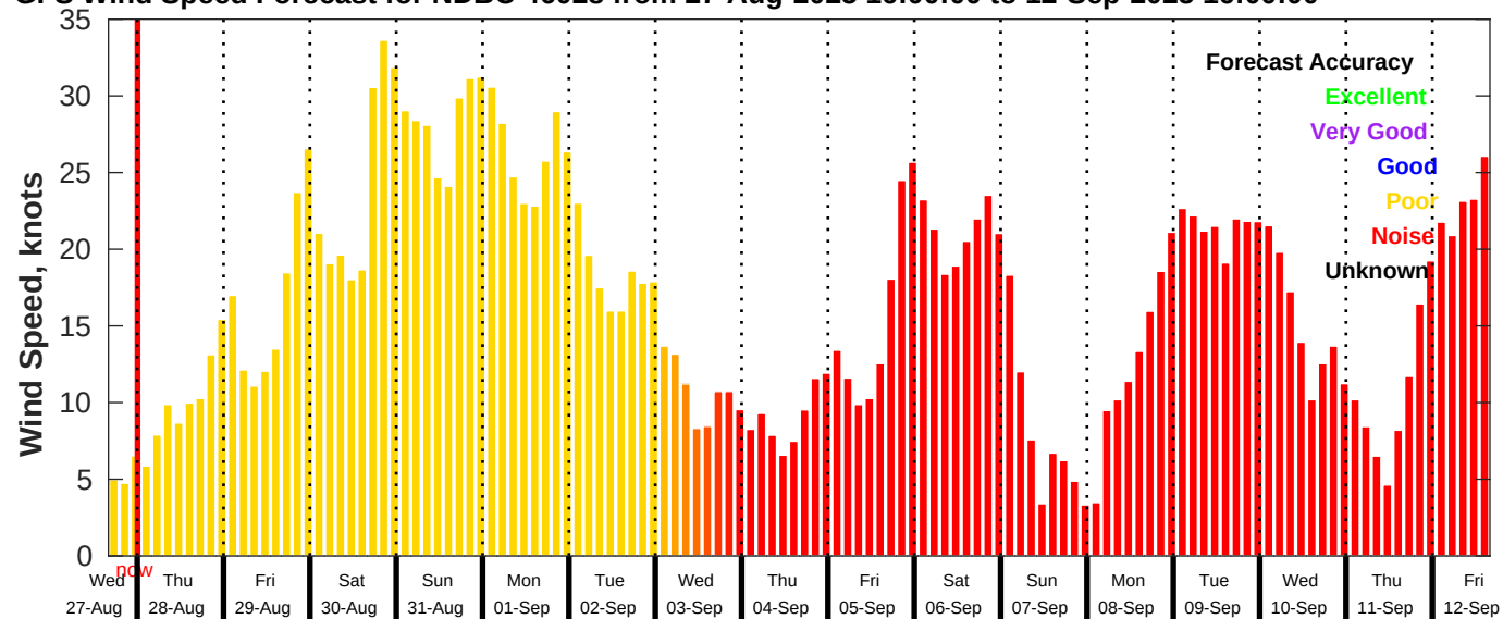
GFS Wind Speed Forecast for NDBC 46028 from 27-Aug-2025 16:00:00 to 12-Sep-2025 16:00:00
