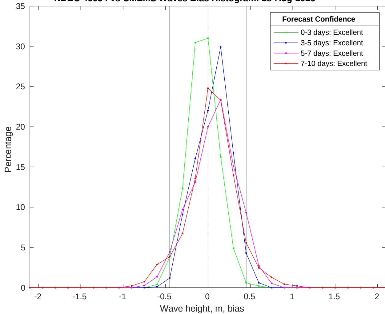
NDBC 46054 vs CMEMS Waves Bias Histogram: 28-Aug-2025
