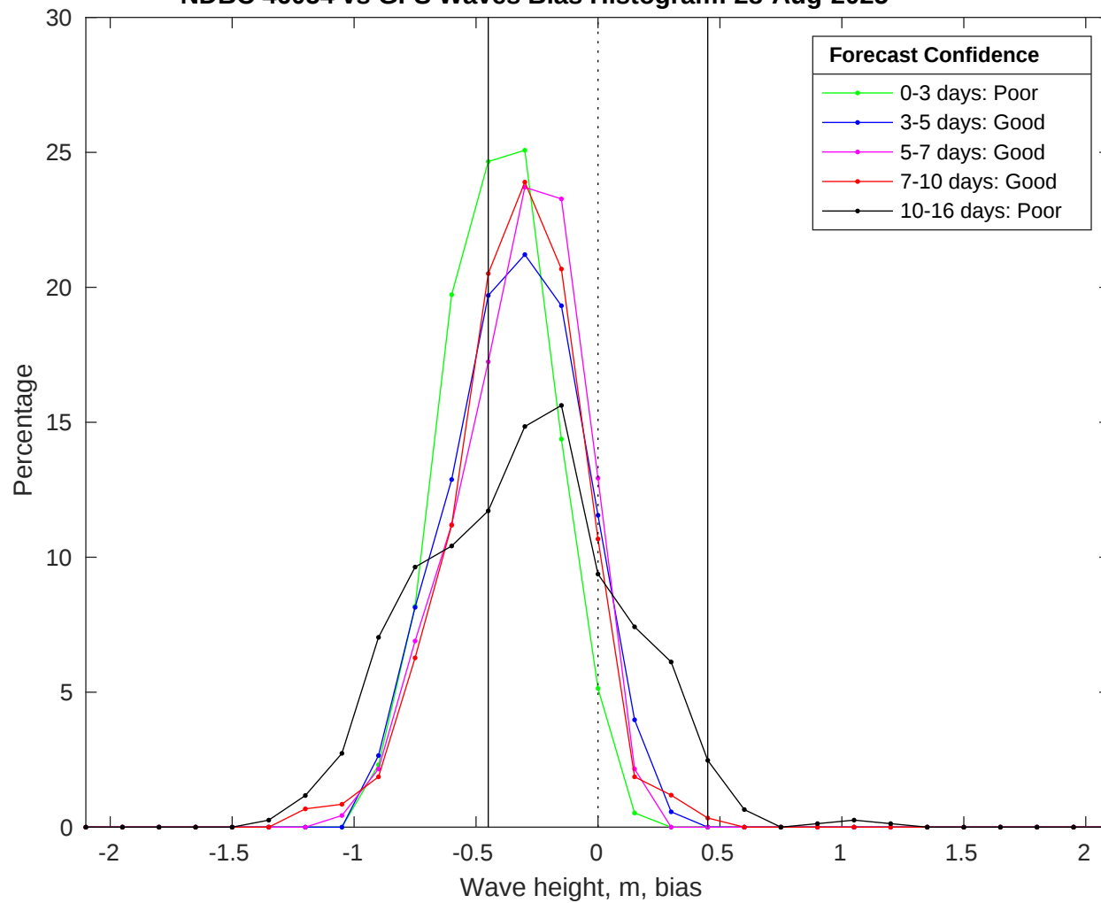
NDBC 46054 vs GFS Waves Bias Histogram: 28-Aug-2025
