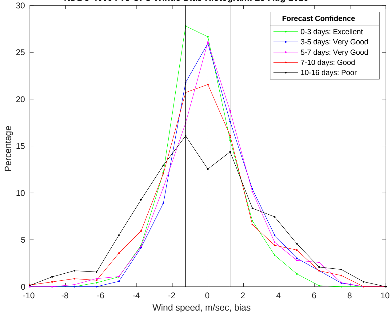
NDBC 46054 vs GFS Winds Bias Histogram: 28-Aug-2025
