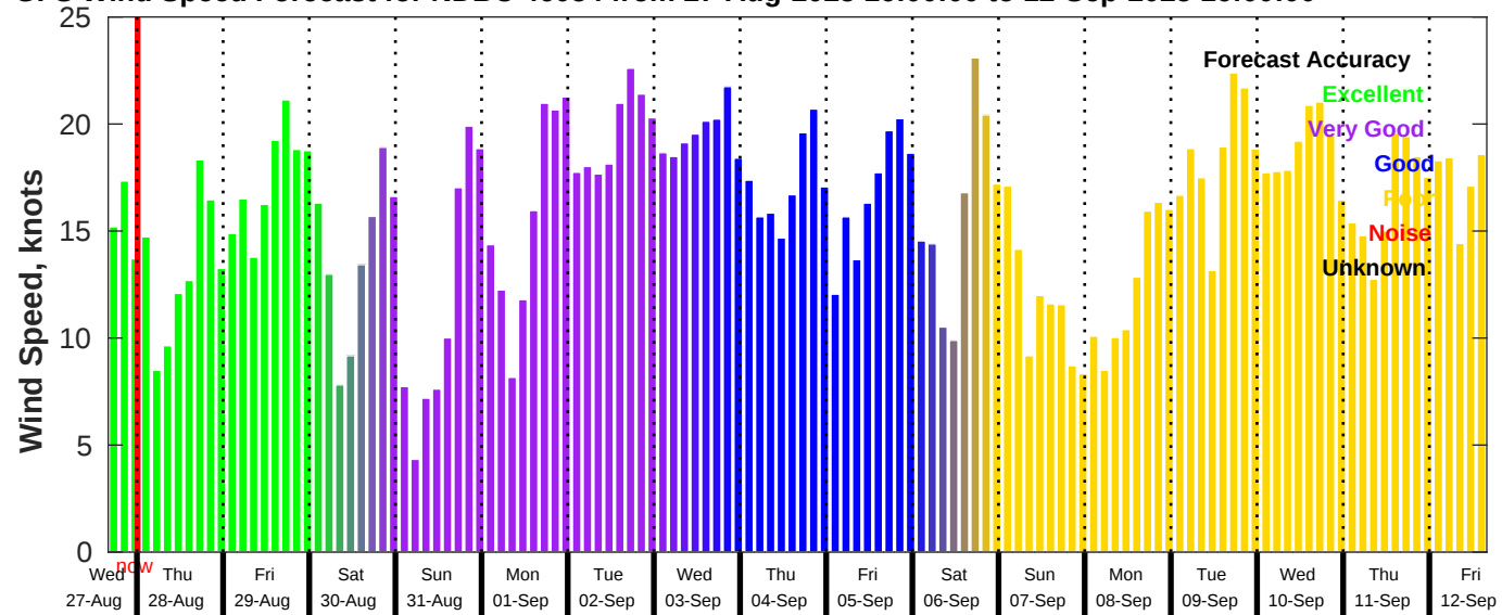
GFS Wind Speed Forecast for NDBC 46054 from 27-Aug-2025 16:00:00 to 12-Sep-2025 16:00:00
