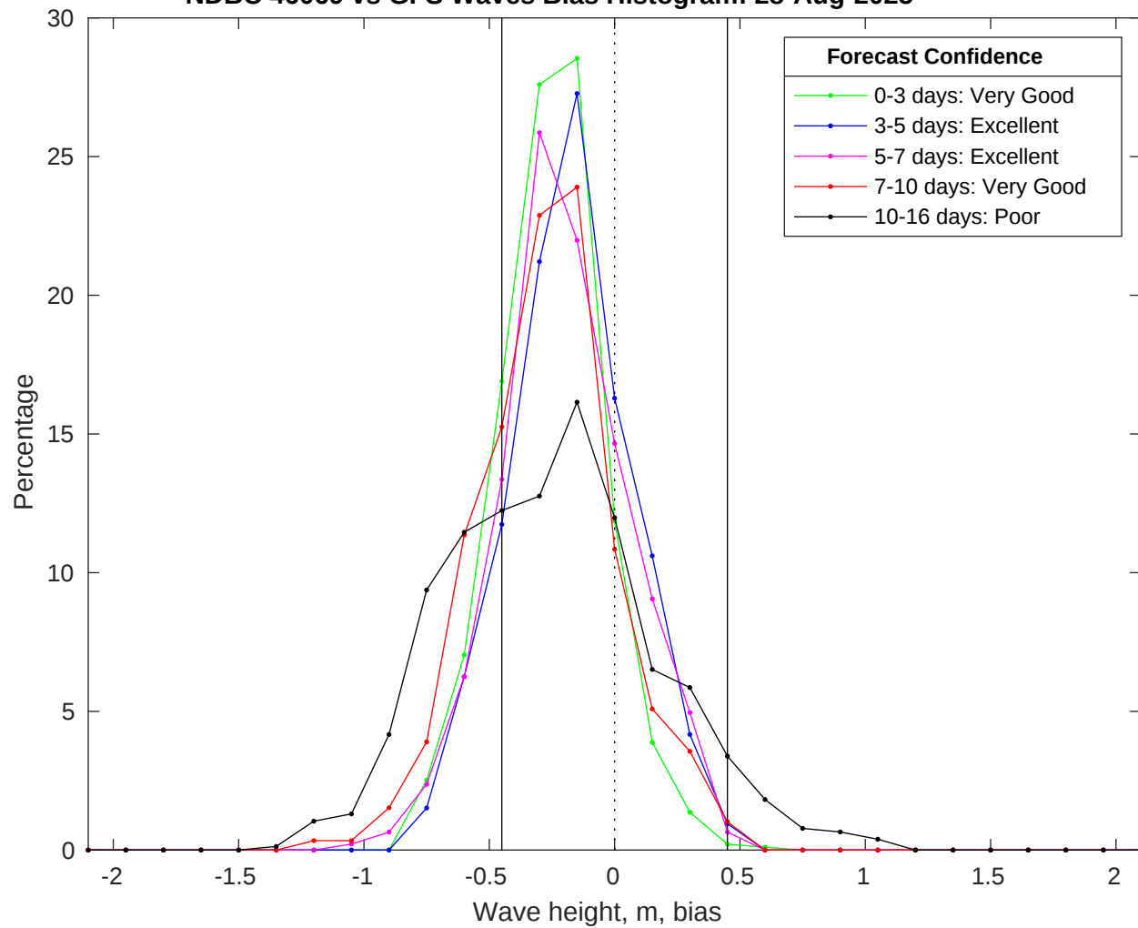
NDBC 46069 vs GFS Waves Bias Histogram: 28-Aug-2025
