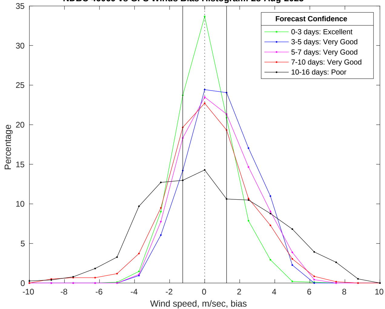
NDBC 46069 vs GFS Winds Bias Histogram: 28-Aug-2025
