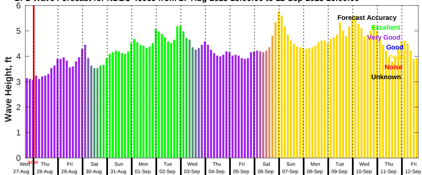
GFS Wave Forecast for NDBC 46069 from 27-Aug-2025 16:00:00 to 12-Sep-2025 16:00:00
