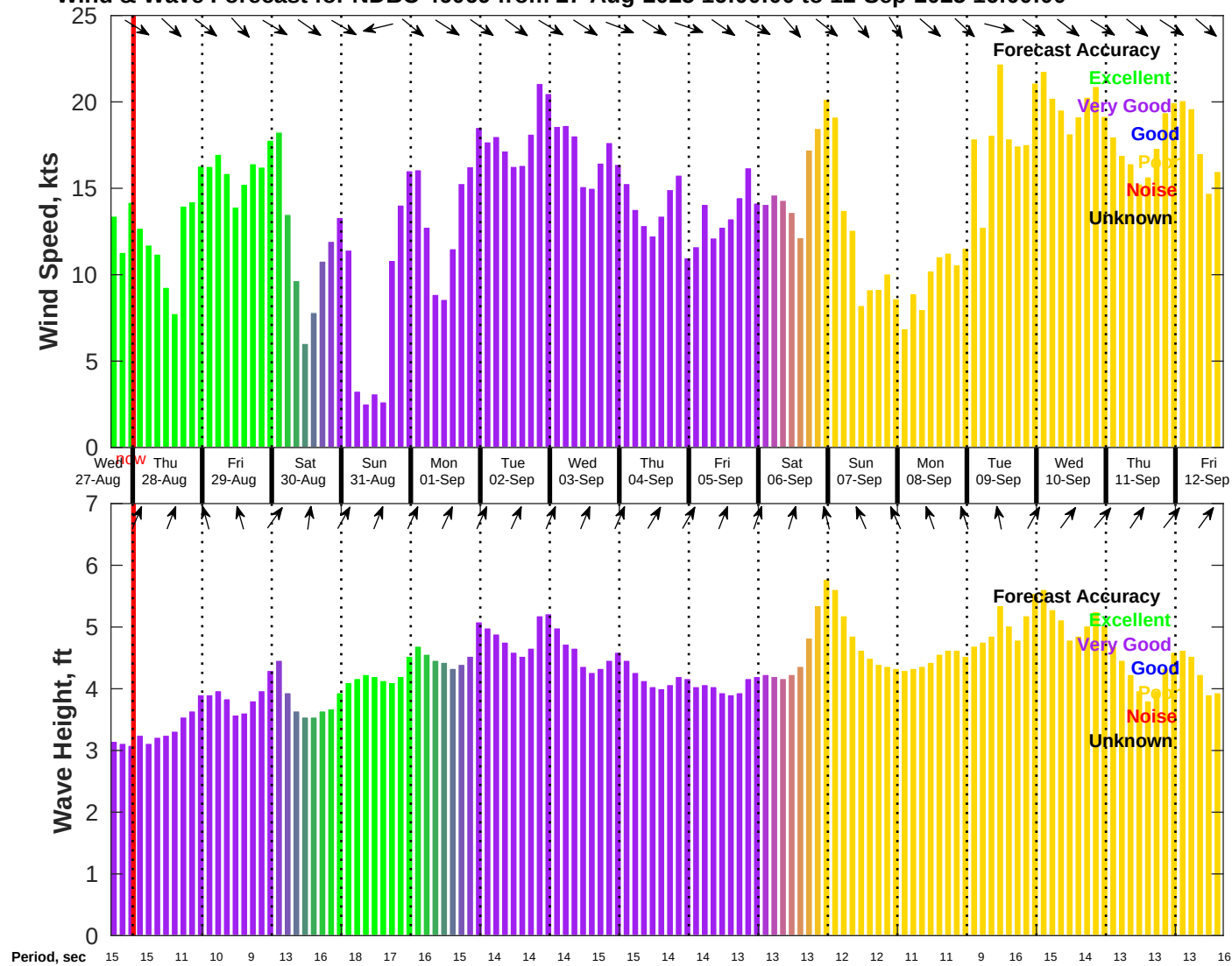
Wind & Wave Forecast for NDBC 46069 from 27-Aug-2025 16:00:00 to 12-Sep-2025 16:00:00
