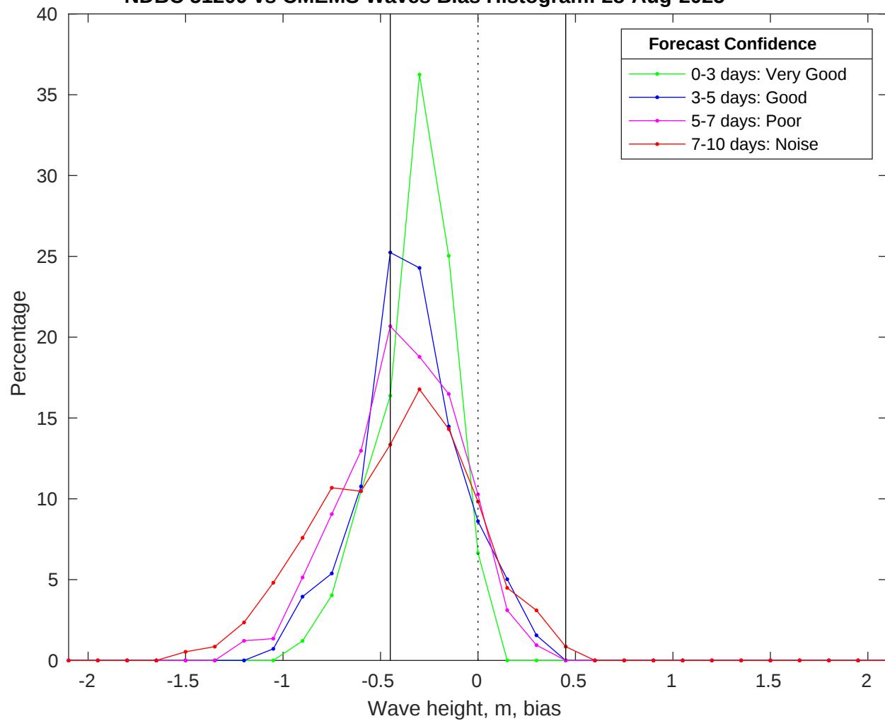
NDBC 51209 vs CMEMS Waves Bias Histogram: 28-Aug-2025
