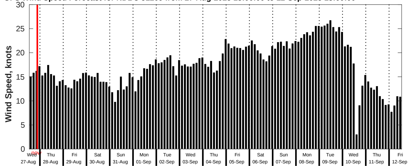
GFS Wind Speed Forecast for NDBC 51209 from 27-Aug-2025 13:00:00 to 12-Sep-2025 13:00:00
