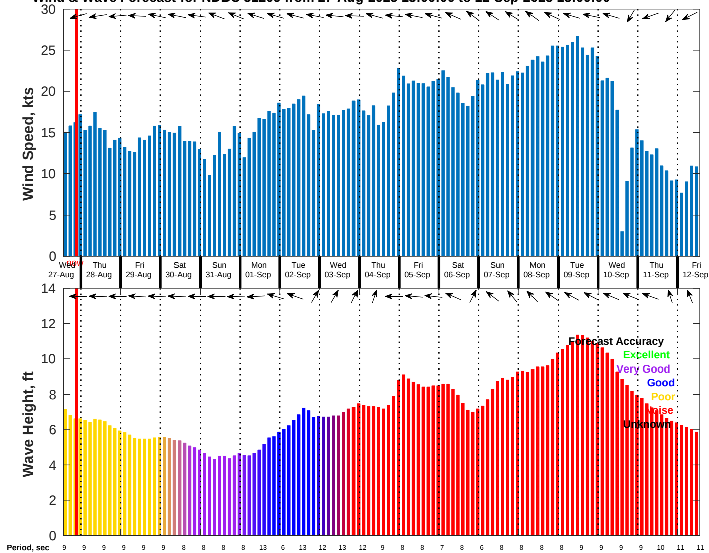
Wind & Wave Forecast for NDBC 51209 from 27-Aug-2025 13:00:00 to 12-Sep-2025 13:00:00
