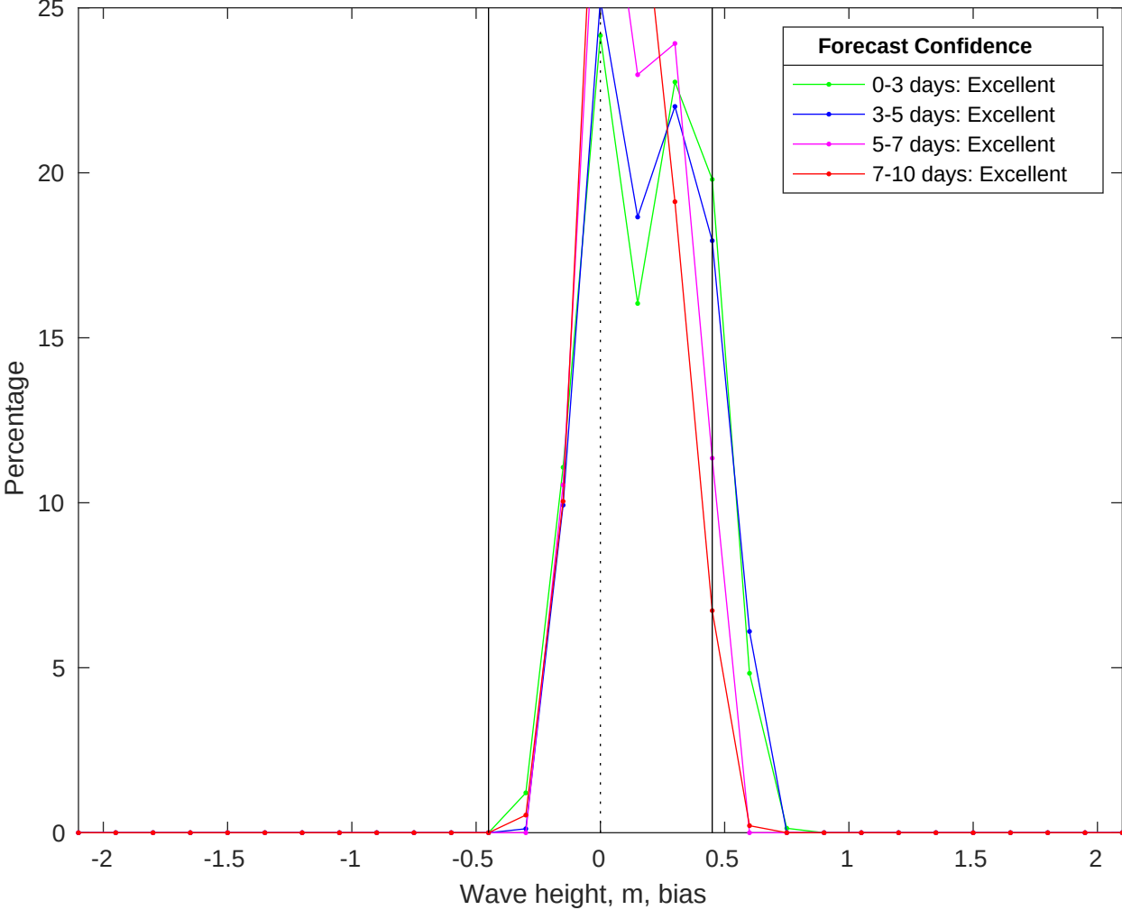
NDBC 51211 vs CMEMS Waves Bias Histogram: 28-Aug-2025
