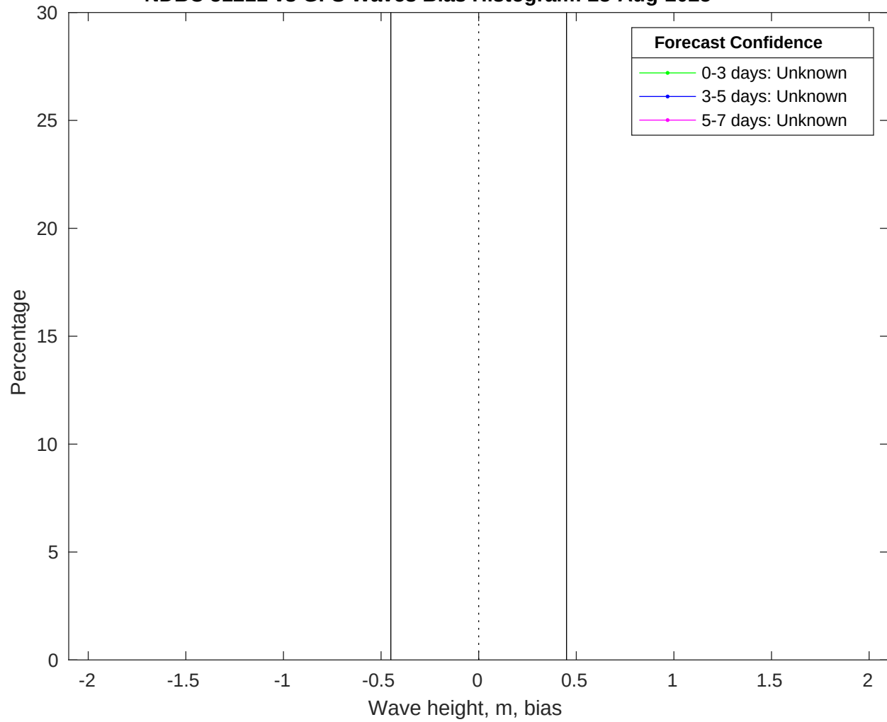
NDBC 51211 vs GFS Waves Bias Histogram: 28-Aug-2025
