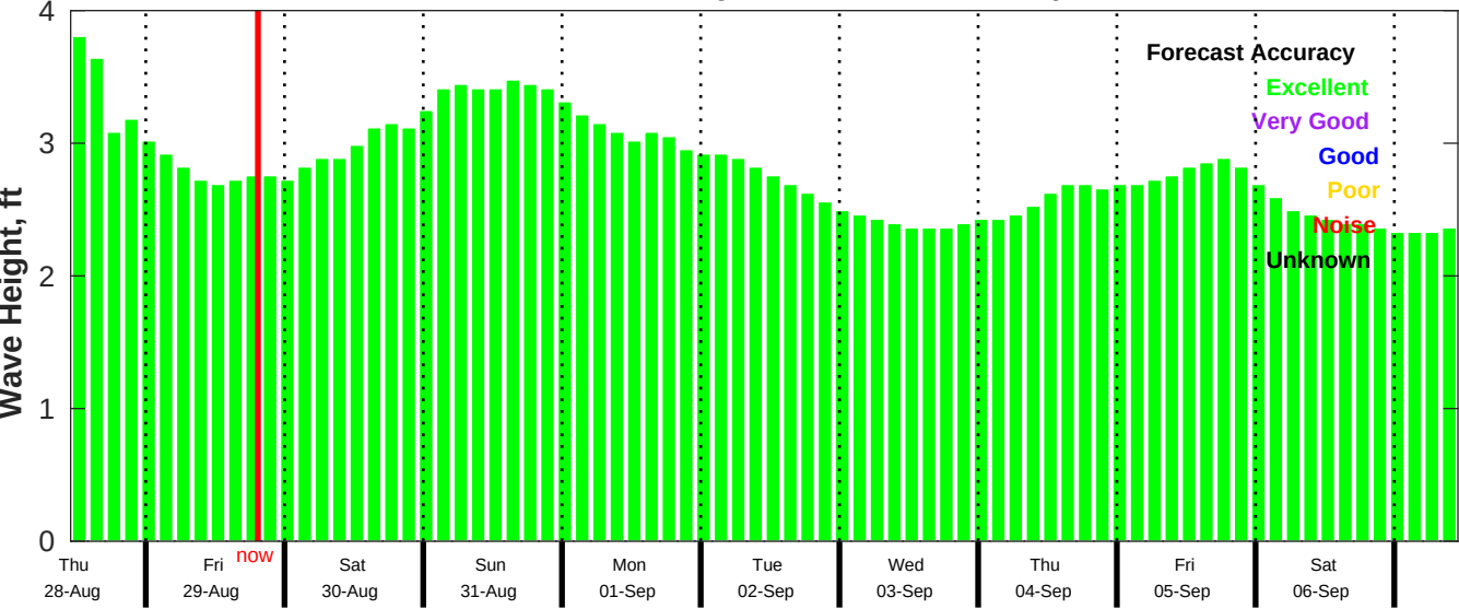
CMEMS Wave Forecast for NDBC 52211 from 27-Aug-2025 11:00:00 to 06-Sep-2025 11:00:00
