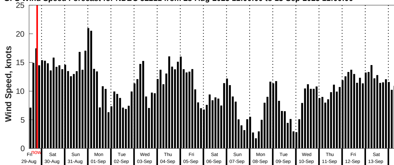
GFS Wind Speed Forecast for NDBC 52211 from 28-Aug-2025 11:00:00 to 13-Sep-2025 11:00:00
