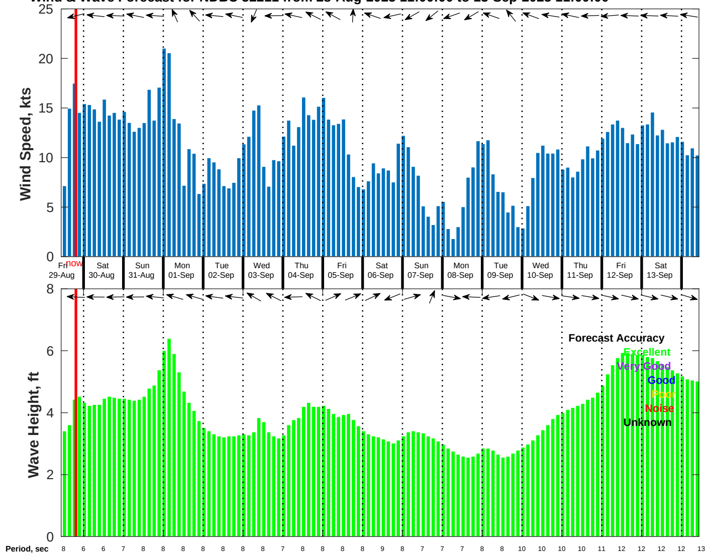
Wind & Wave Forecast for NDBC 52211 from 28-Aug-2025 11:00:00 to 13-Sep-2025 11:00:00
