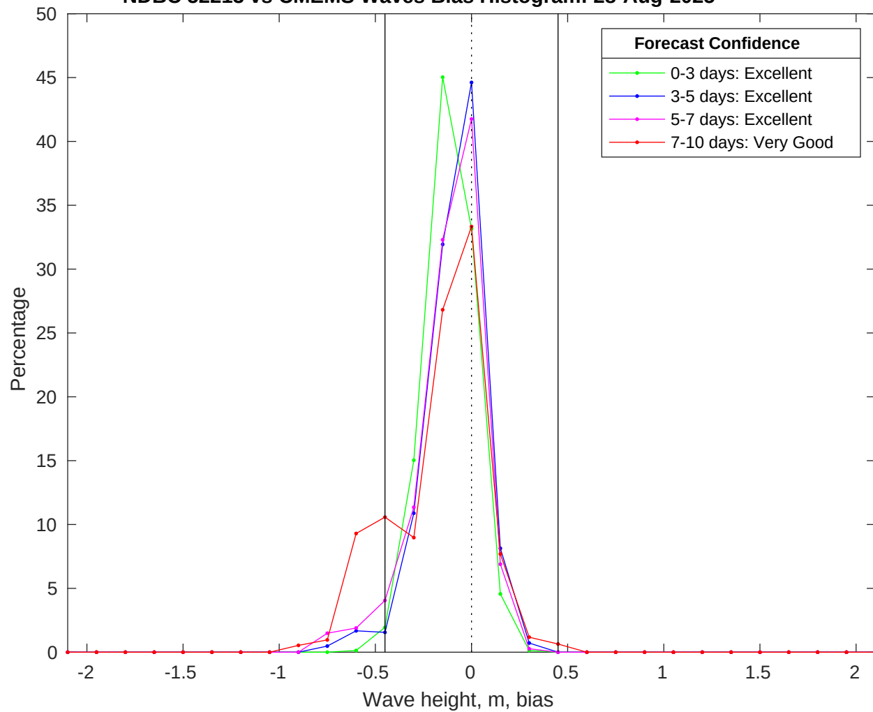
NDBC 52213 vs CMEMS Waves Bias Histogram: 28-Aug-2025
