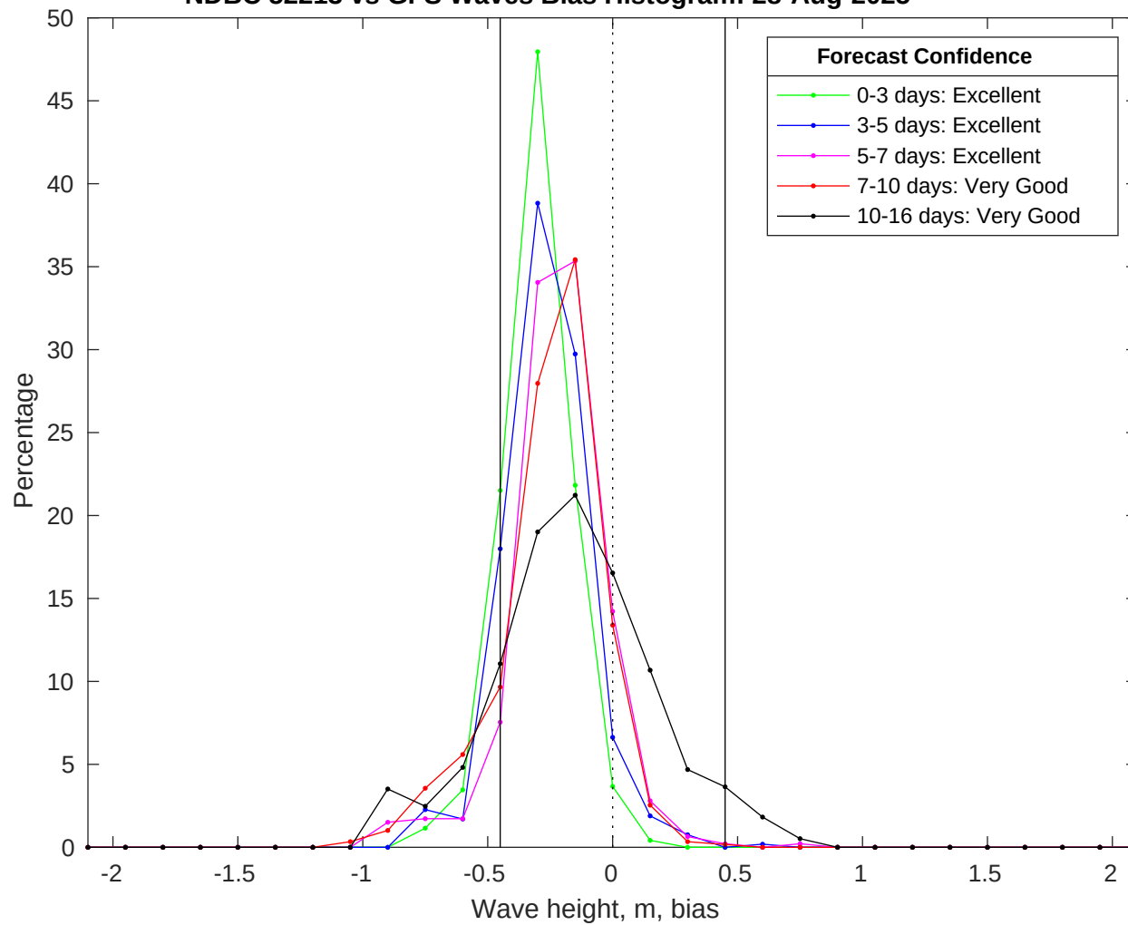
NDBC 52213 vs GFS Waves Bias Histogram: 28-Aug-2025
