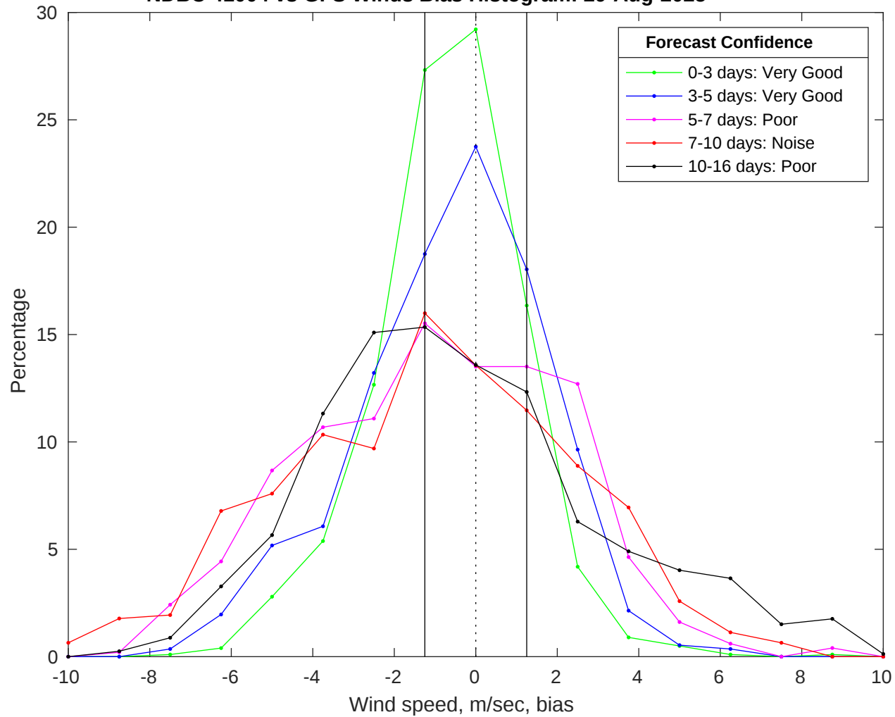
NDBC 41004 vs GFS Winds Bias Histogram: 29-Aug-2025
