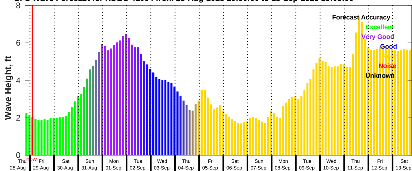
GFS Wave Forecast for NDBC 41004 from 28-Aug-2025 19:00:00 to 13-Sep-2025 19:00:00
