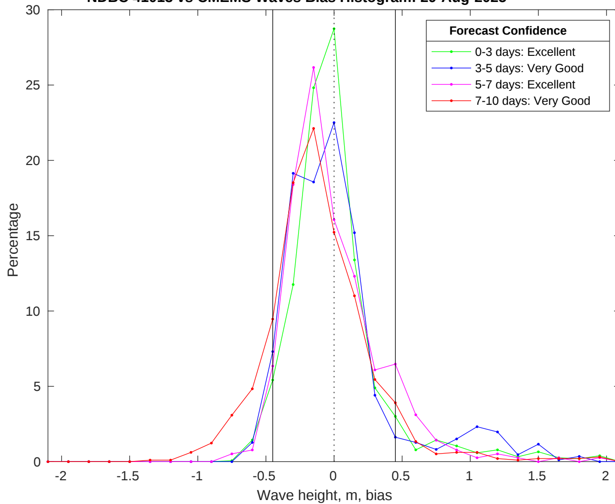
NDBC 41013 vs CMEMS Waves Bias Histogram: 29-Aug-2025
