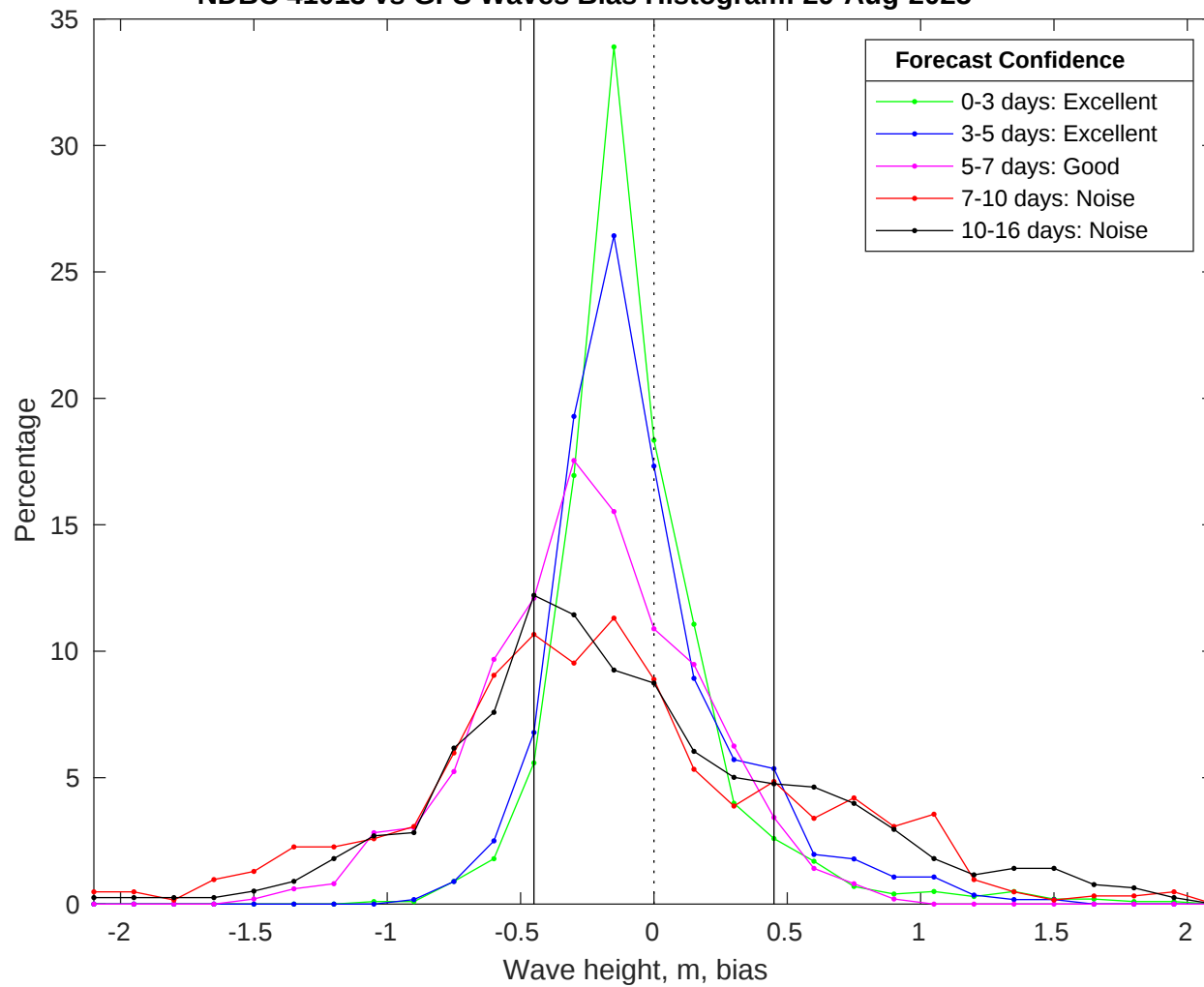
NDBC 41013 vs GFS Waves Bias Histogram: 29-Aug-2025
