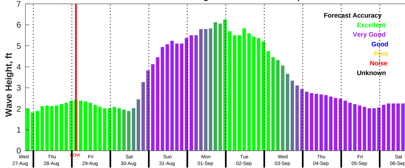
CMEMS Wave Forecast for NDBC 41013 from 27-Aug-2025 19:00:00 to 06-Sep-2025 19:00:00
