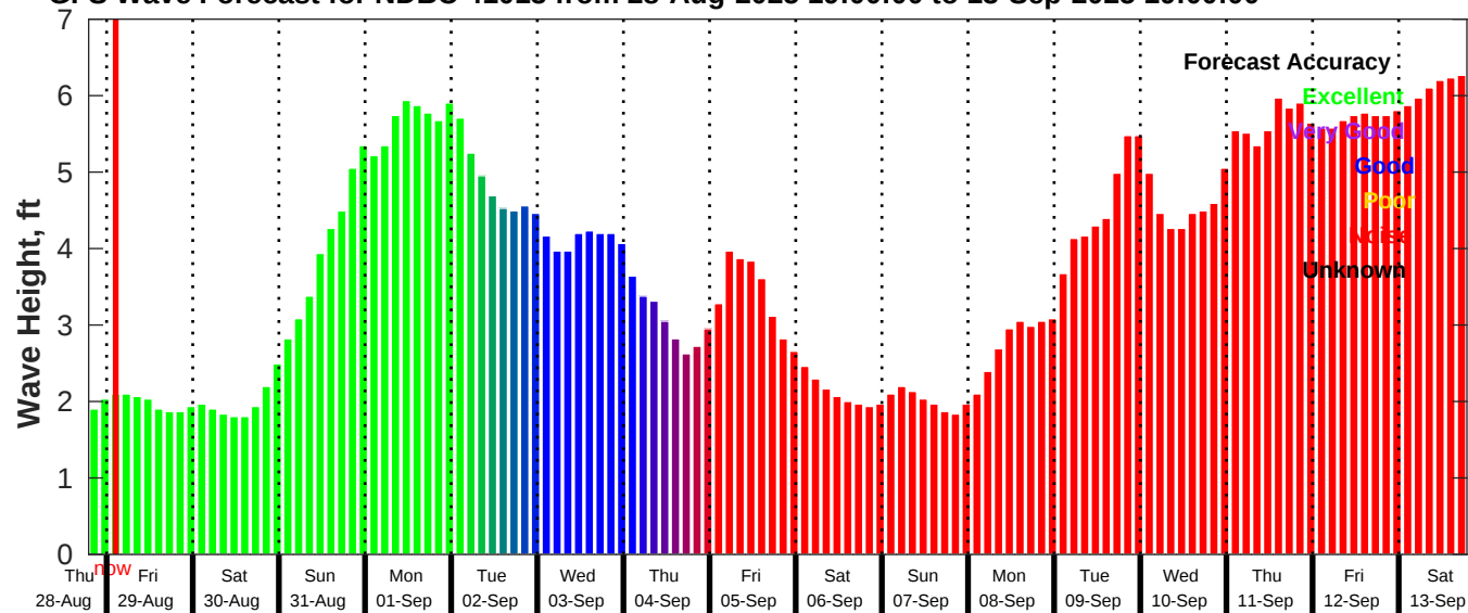
GFS Wave Forecast for NDBC 41013 from 28-Aug-2025 19:00:00 to 13-Sep-2025 19:00:00
