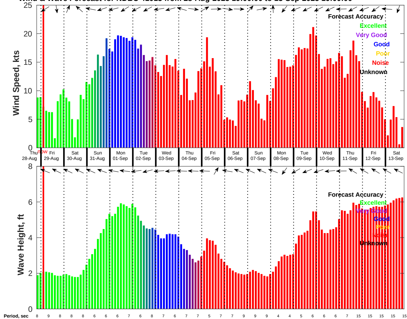
Wind & Wave Forecast for NDBC 41013 from 28-Aug-2025 19:00:00 to 13-Sep-2025 19:00:00
