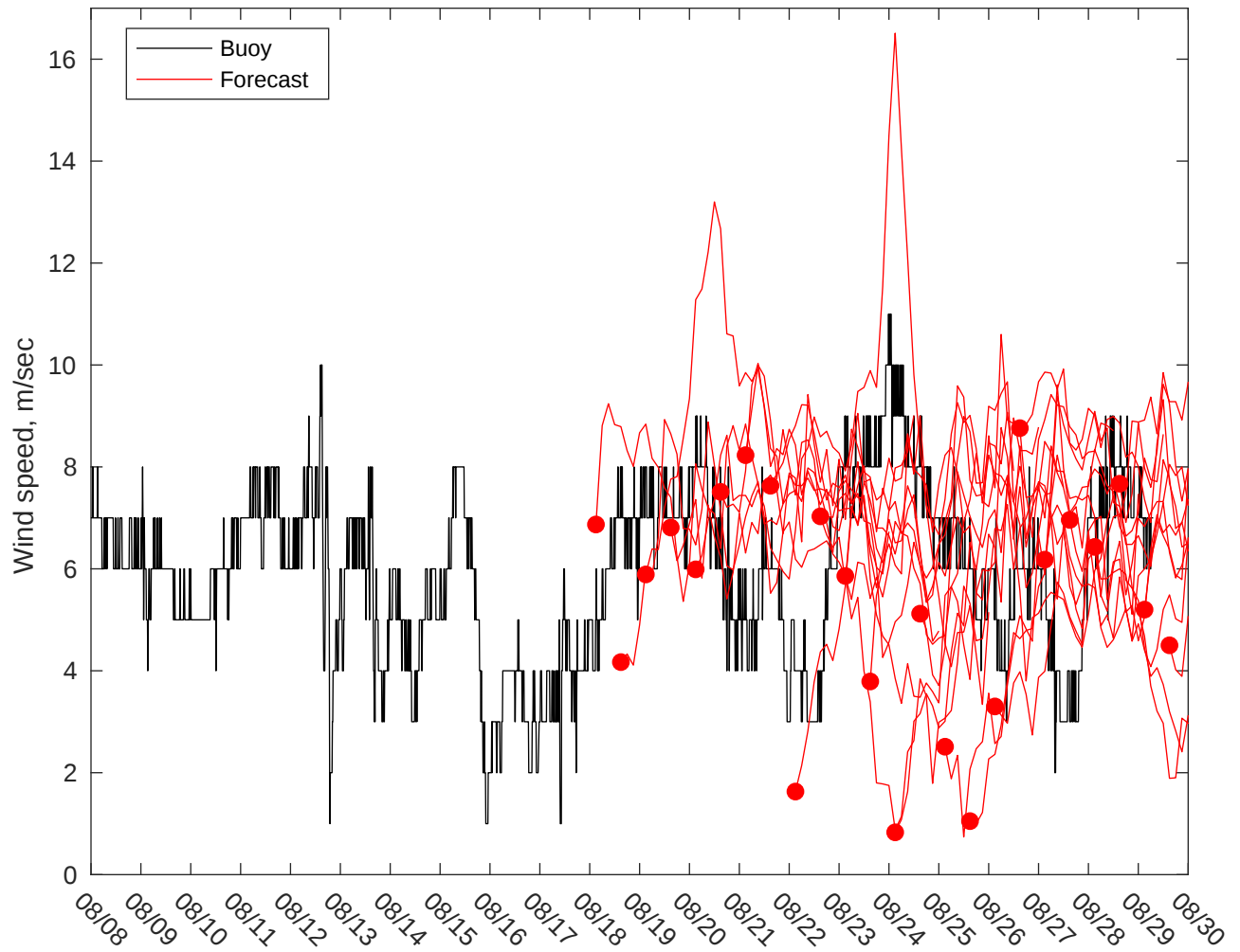
NDBC 41040 vs GFS Winds: 10 to 16 day forecast
