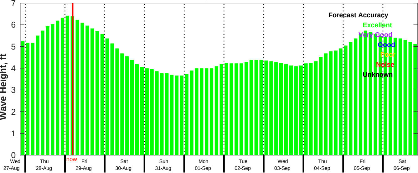
CMEMS Wave Forecast for NDBC 41040 from 27-Aug-2025 21:00:00 to 06-Sep-2025 21:00:00
