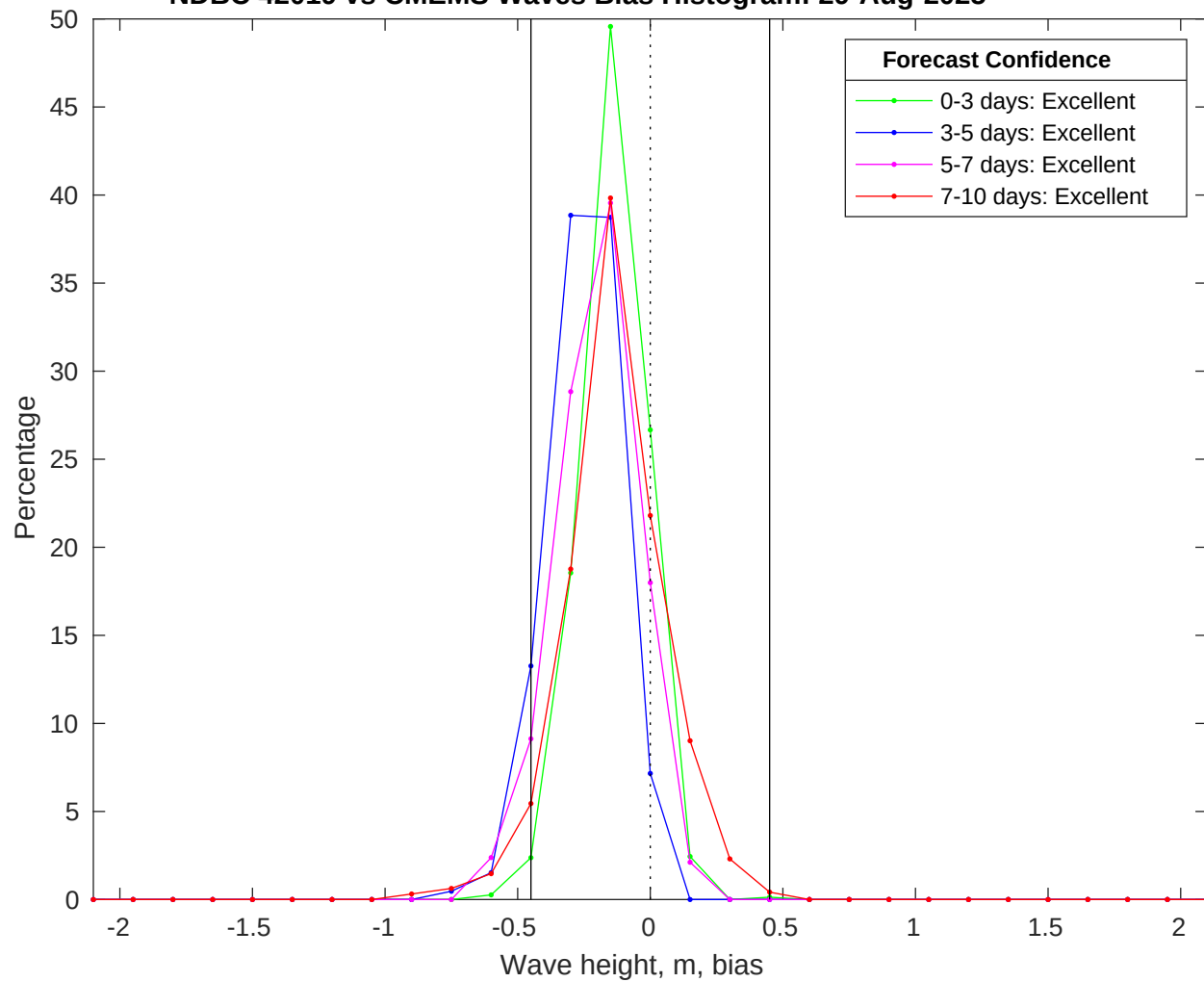
NDBC 42019 vs CMEMS Waves Bias Histogram: 29-Aug-2025
