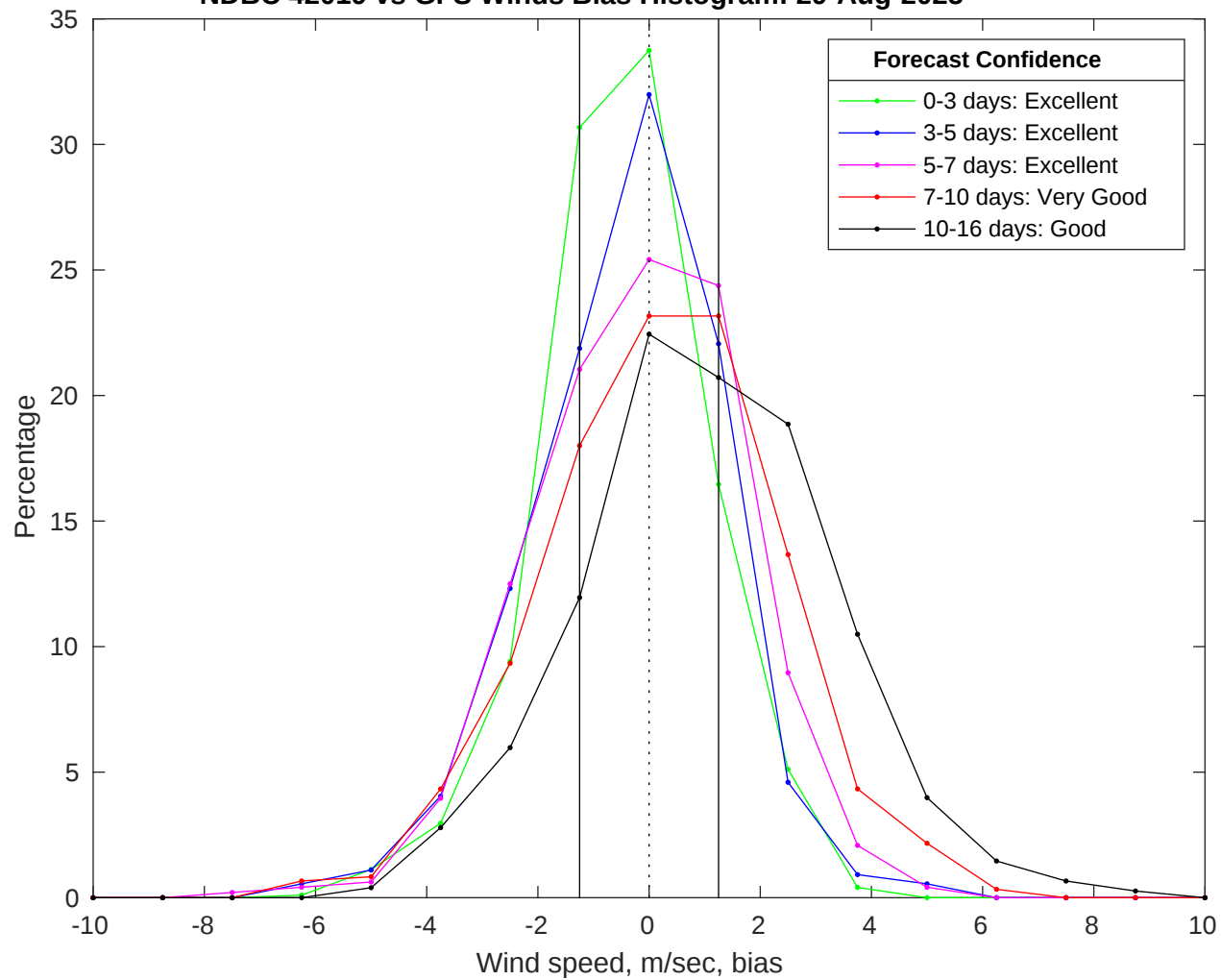
NDBC 42019 vs GFS Winds Bias Histogram: 29-Aug-2025
