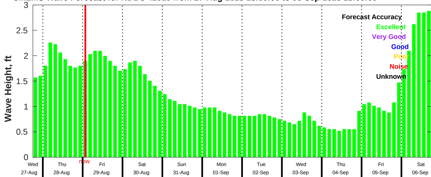
CMEMS Wave Forecast for NDBC 42019 from 27-Aug-2025 18:00:00 to 06-Sep-2025 18:00:00
