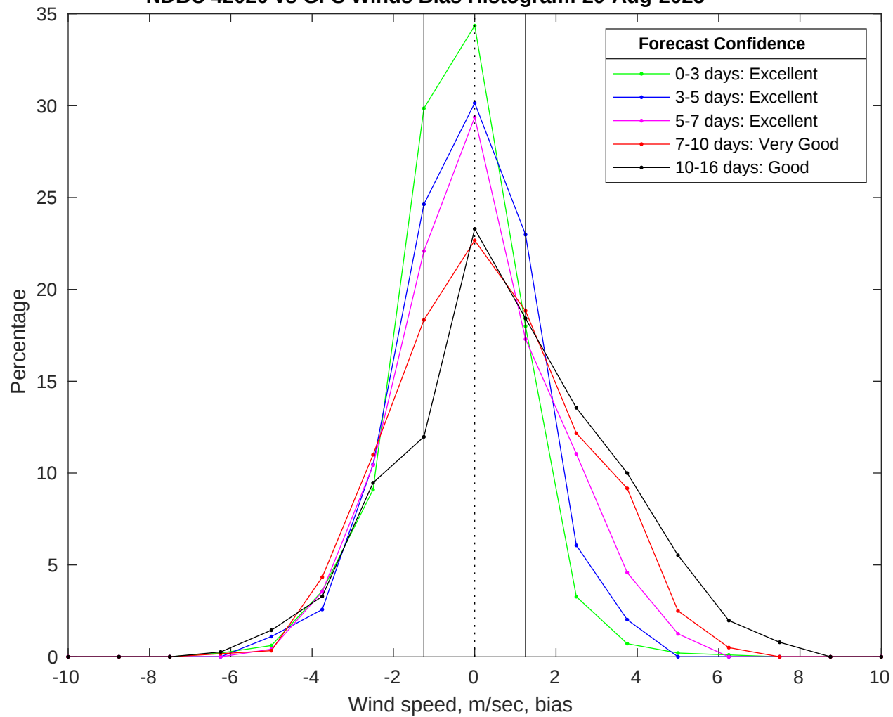
NDBC 42020 vs GFS Winds Bias Histogram: 29-Aug-2025
