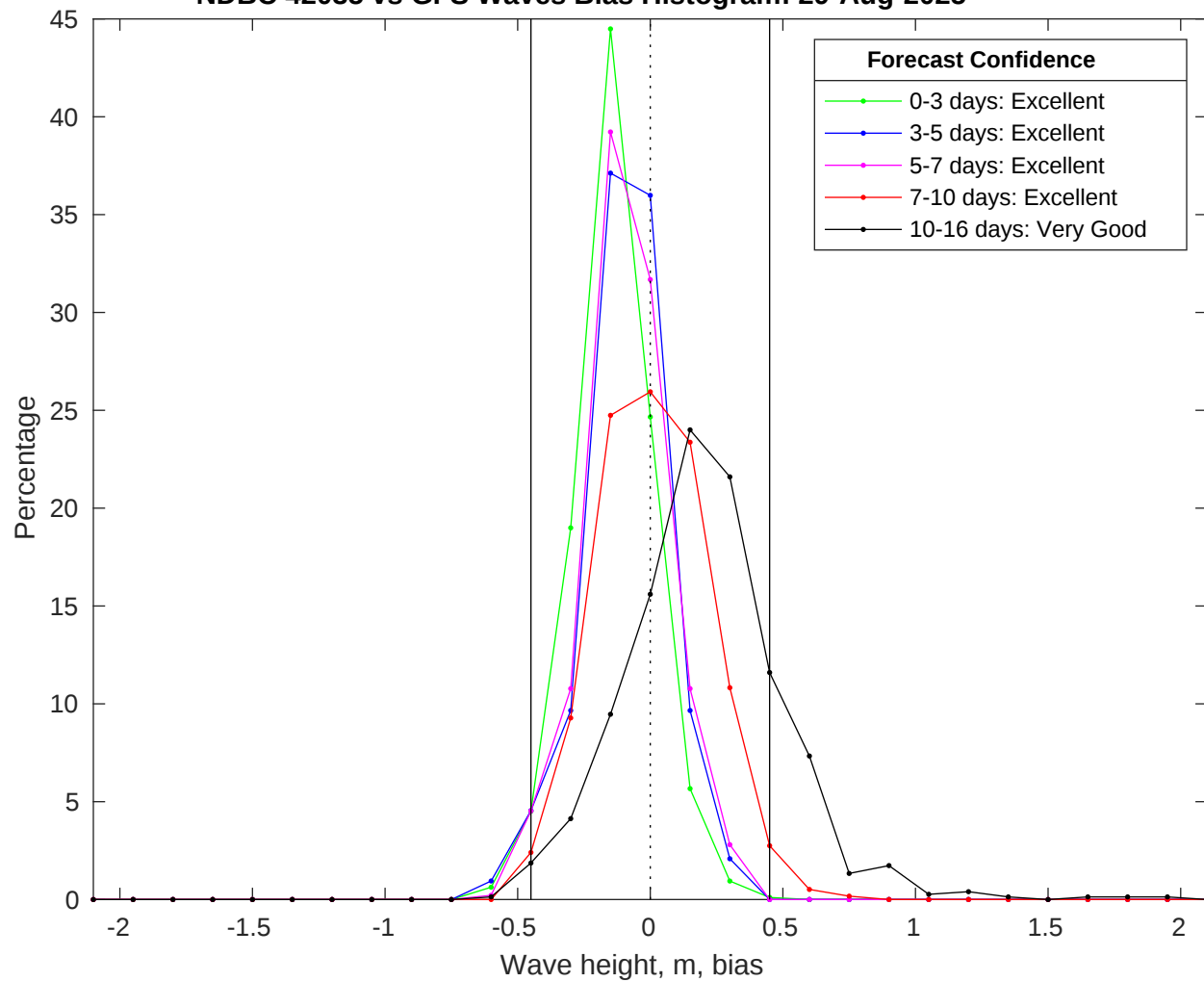
NDBC 42035 vs GFS Waves Bias Histogram: 29-Aug-2025
