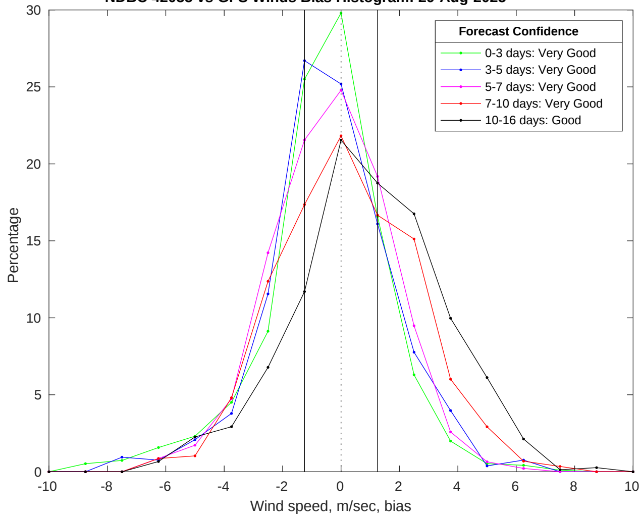
NDBC 42035 vs GFS Winds Bias Histogram: 29-Aug-2025
