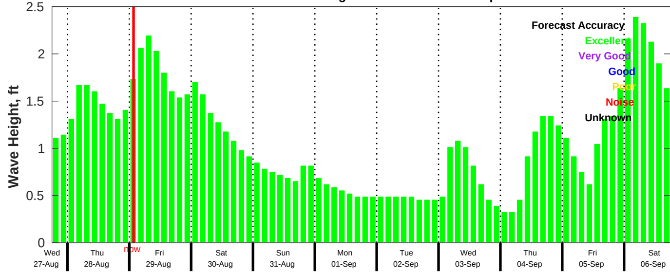
CMEMS Wave Forecast for NDBC 42035 from 27-Aug-2025 18:00:00 to 06-Sep-2025 18:00:00
