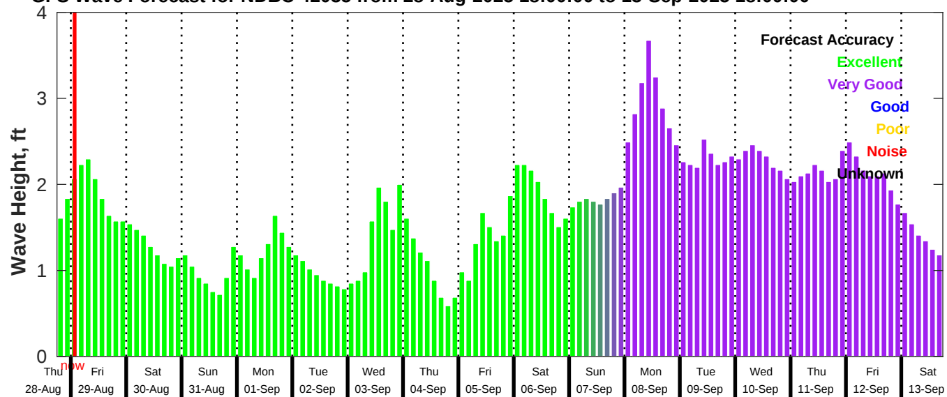
GFS Wave Forecast for NDBC 42035 from 28-Aug-2025 18:00:00 to 13-Sep-2025 18:00:00
