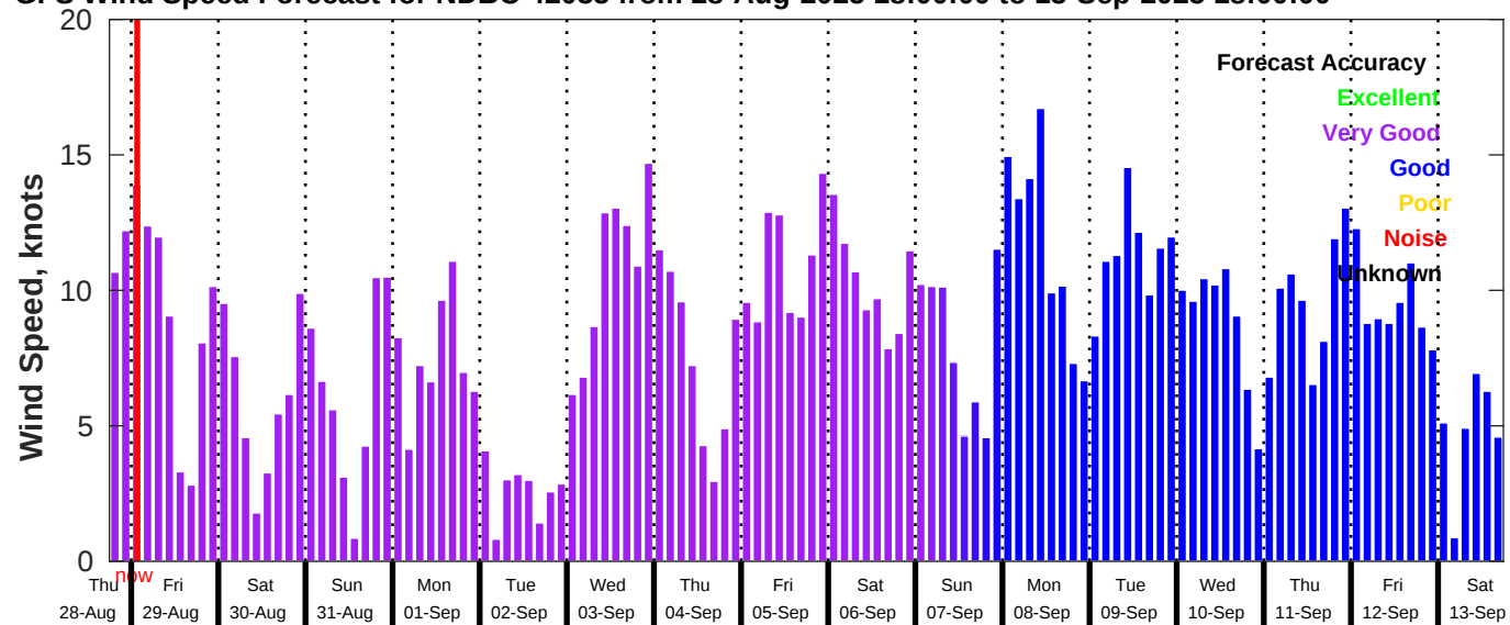
GFS Wind Speed Forecast for NDBC 42035 from 28-Aug-2025 18:00:00 to 13-Sep-2025 18:00:00
