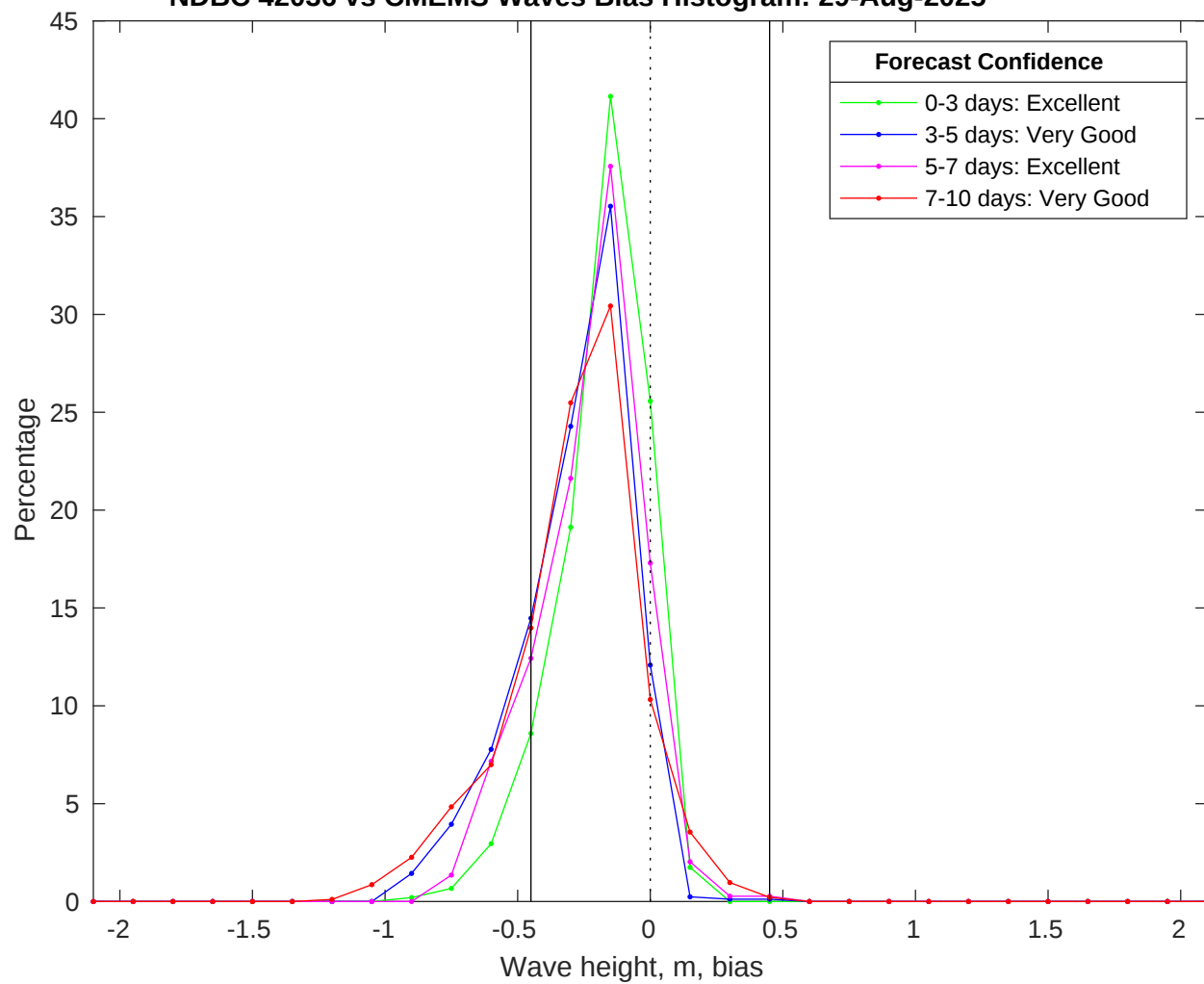
NDBC 42036 vs CMEMS Waves Bias Histogram: 29-Aug-2025
