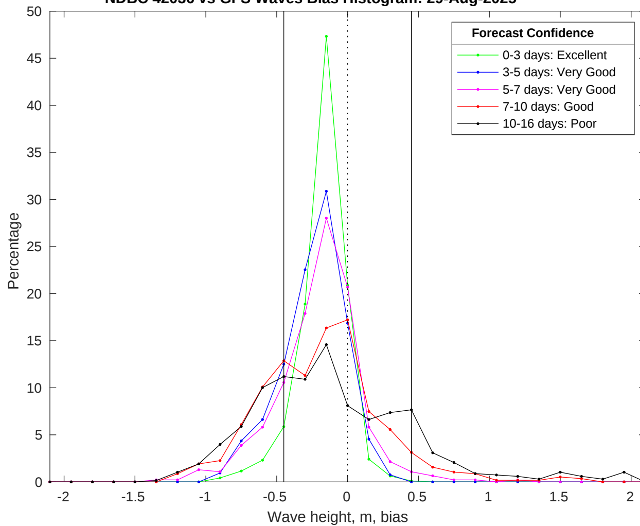
NDBC 42036 vs GFS Waves Bias Histogram: 29-Aug-2025
