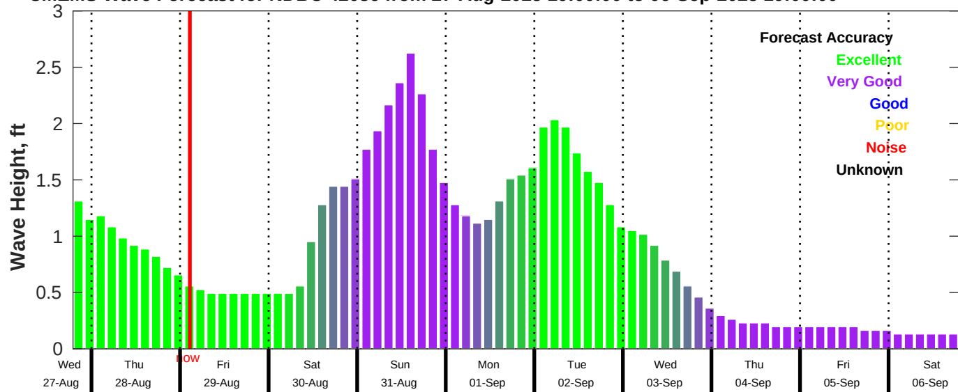
CMEMS Wave Forecast for NDBC 42036 from 27-Aug-2025 19:00:00 to 06-Sep-2025 19:00:00
