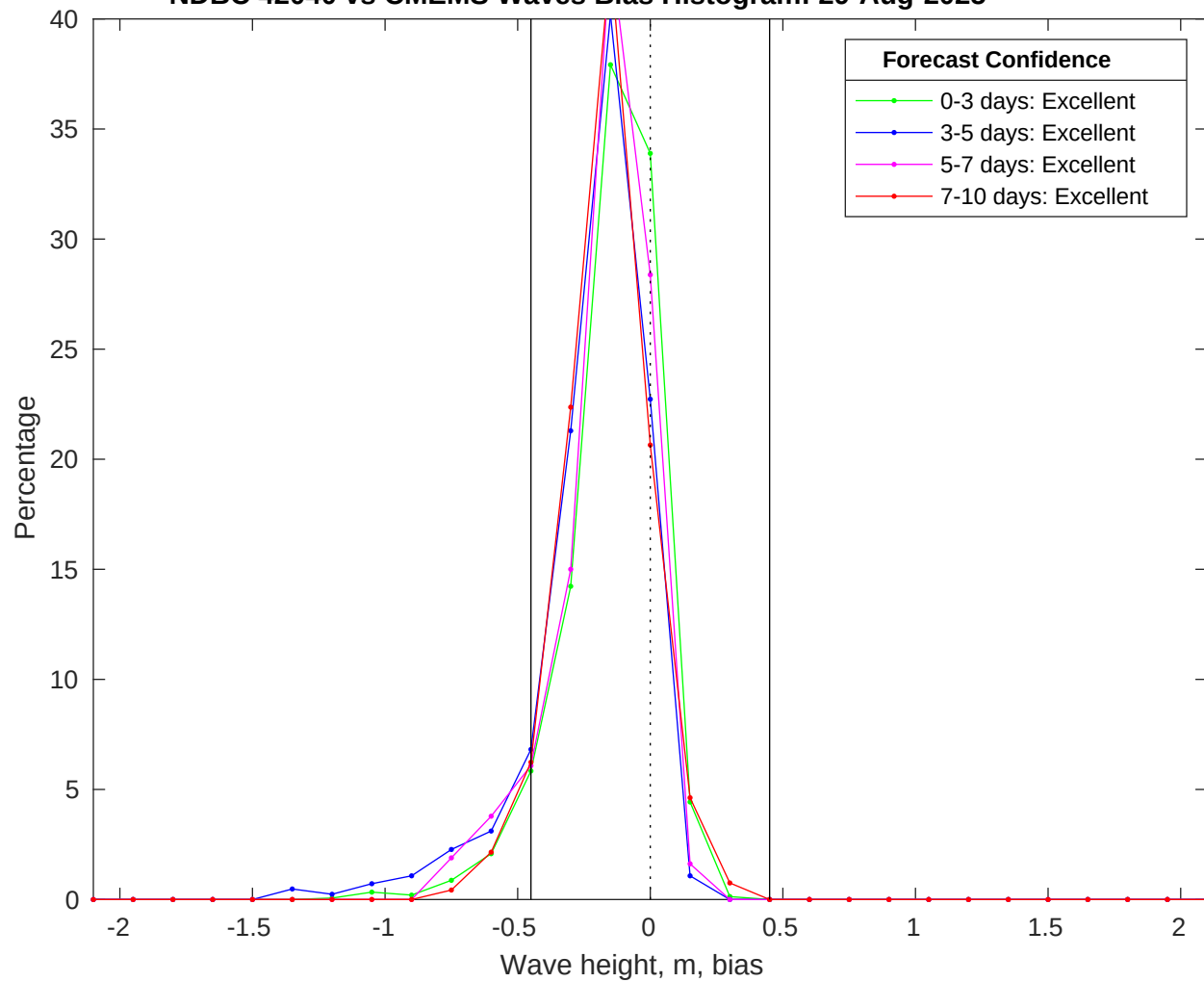
NDBC 42040 vs CMEMS Waves Bias Histogram: 29-Aug-2025
