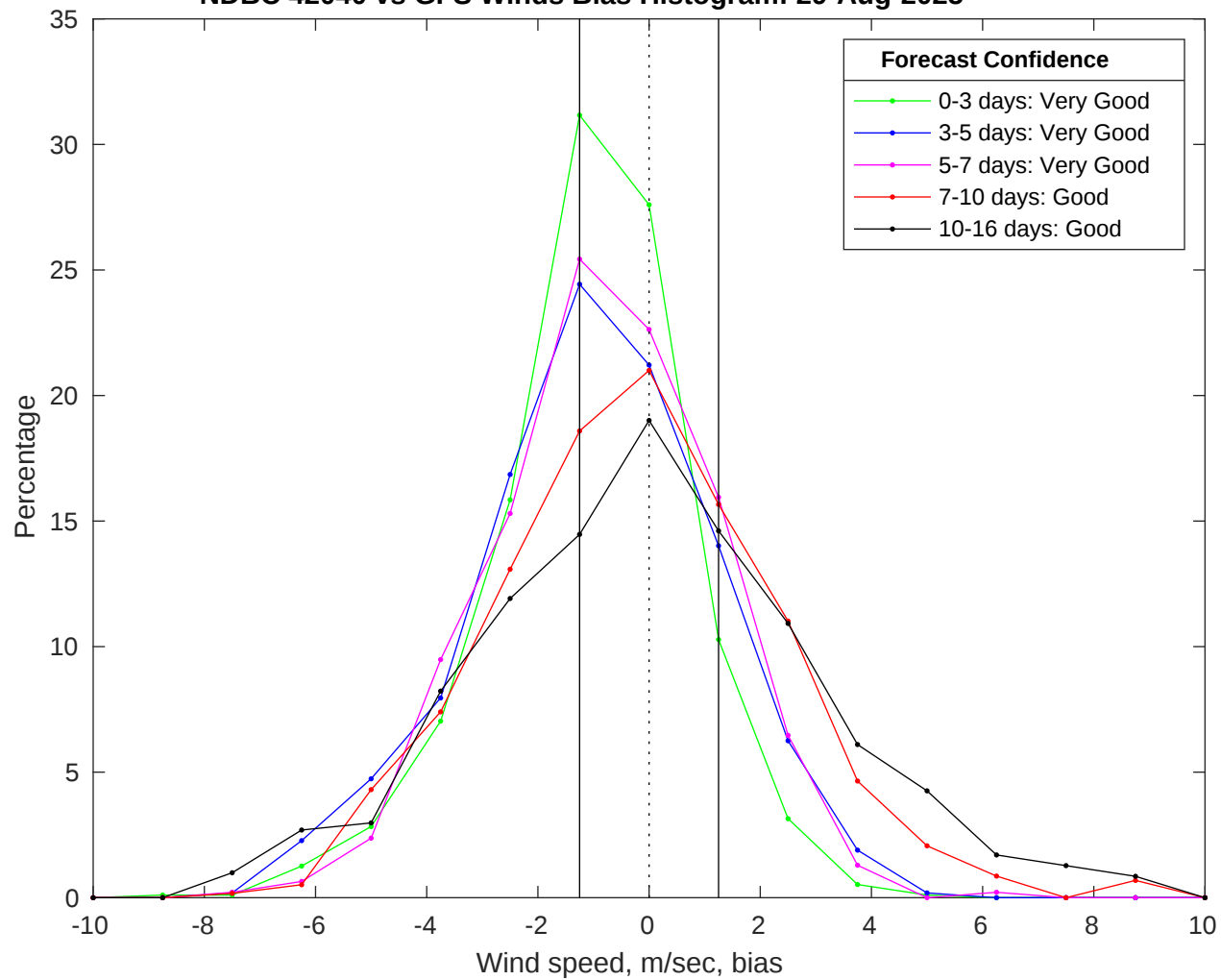
NDBC 42040 vs GFS Winds Bias Histogram: 29-Aug-2025
