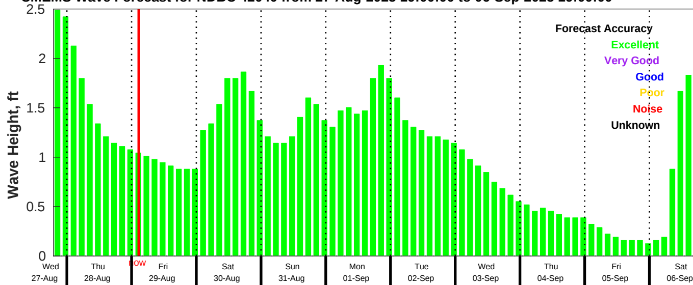
CMEMS Wave Forecast for NDBC 42040 from 27-Aug-2025 19:00:00 to 06-Sep-2025 19:00:00
