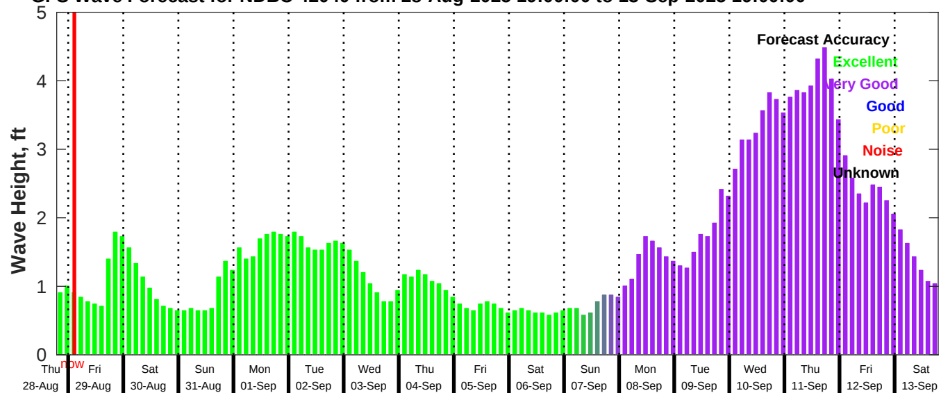
GFS Wave Forecast for NDBC 42040 from 28-Aug-2025 19:00:00 to 13-Sep-2025 19:00:00
