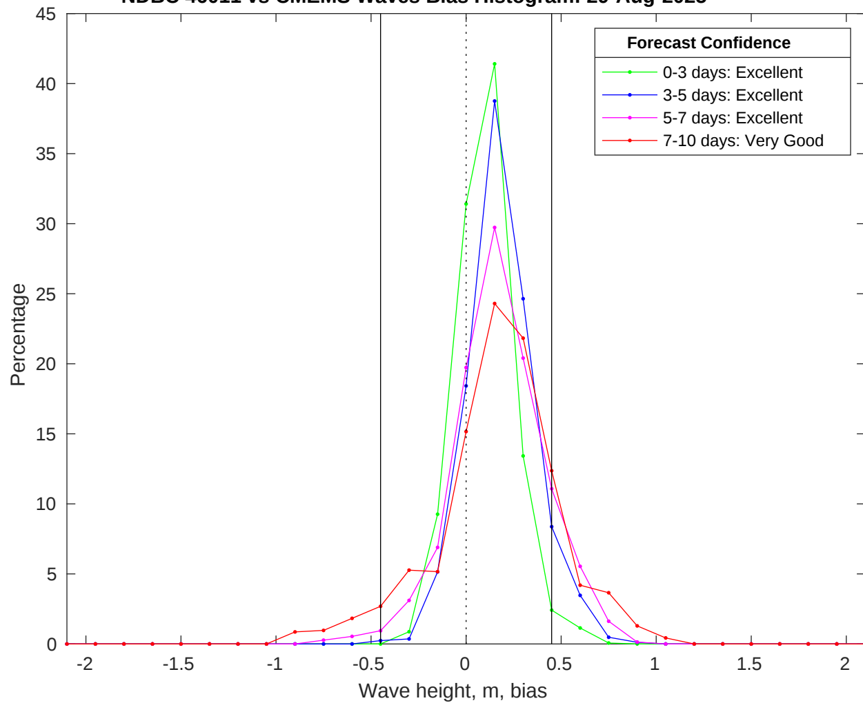
NDBC 46011 vs CMEMS Waves Bias Histogram: 29-Aug-2025
