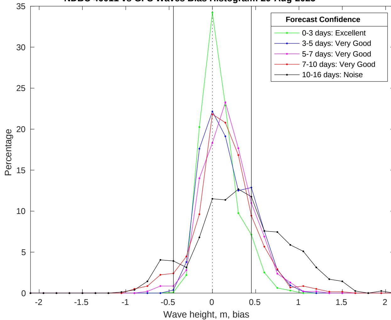
NDBC 46011 vs GFS Waves Bias Histogram: 29-Aug-2025
