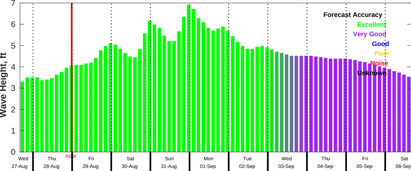
CMEMS Wave Forecast for NDBC 46011 from 27-Aug-2025 16:00:00 to 06-Sep-2025 16:00:00
