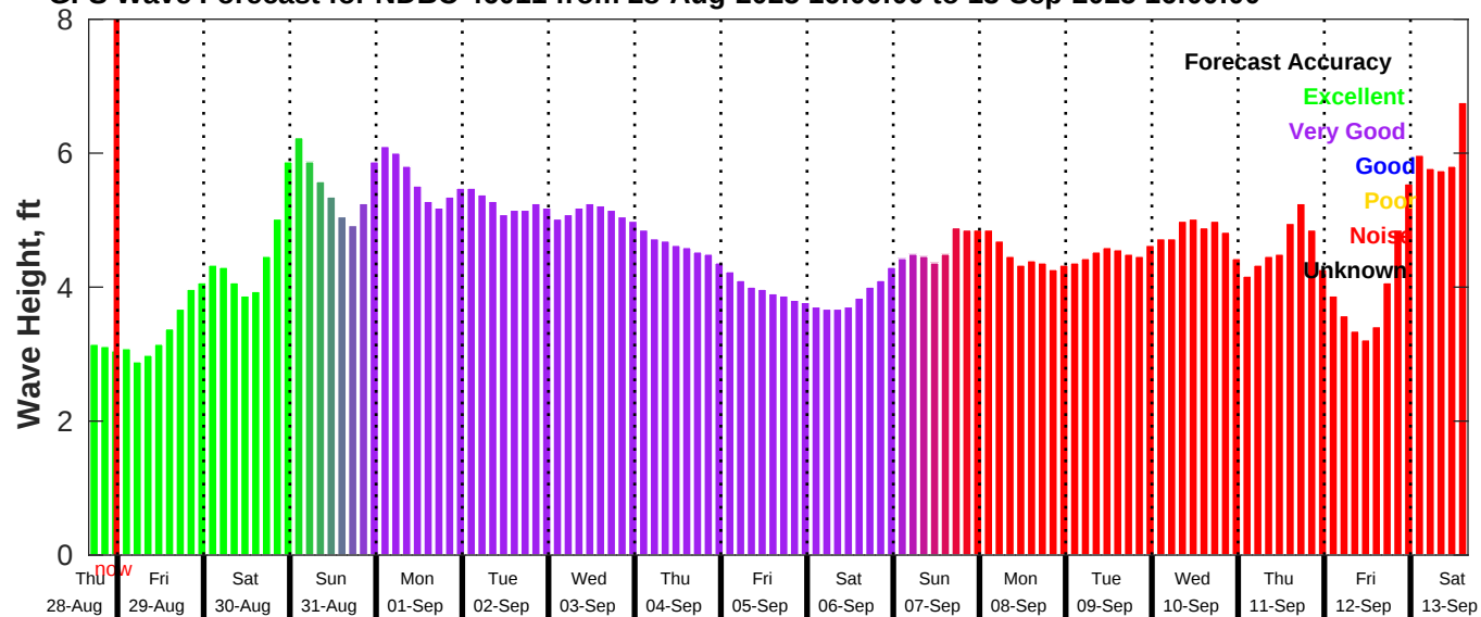
GFS Wave Forecast for NDBC 46011 from 28-Aug-2025 16:00:00 to 13-Sep-2025 16:00:00
