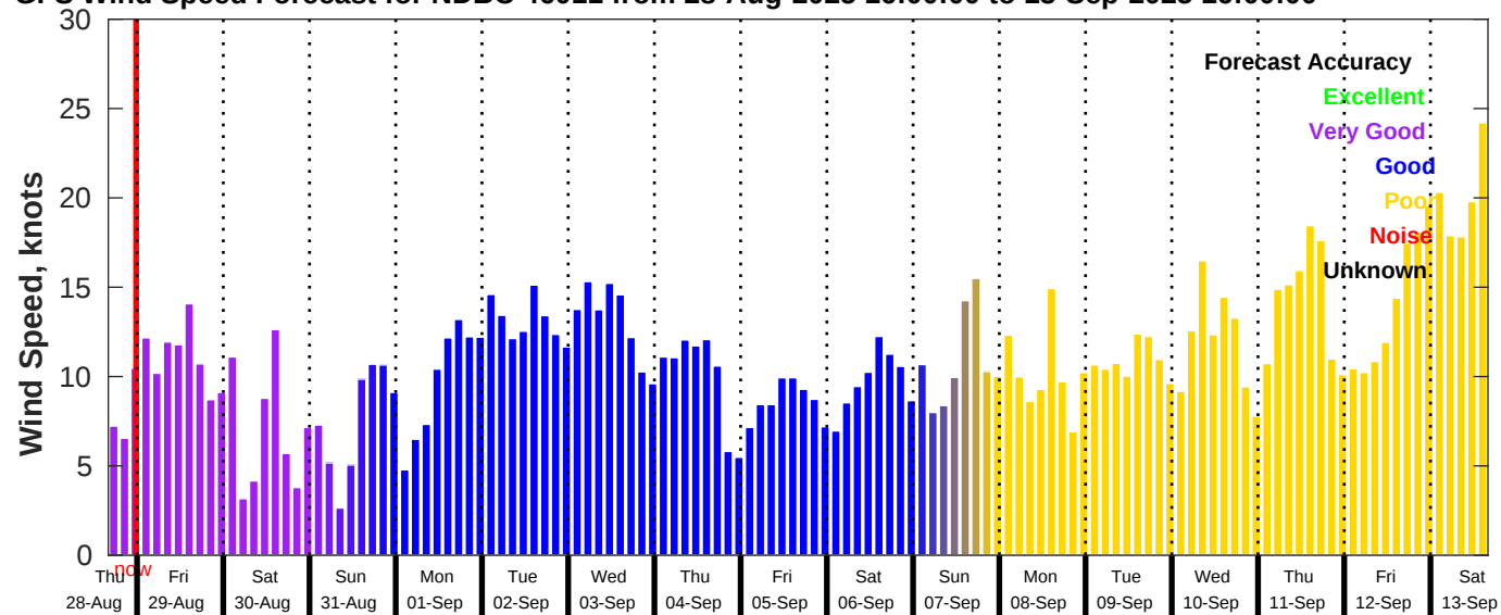
GFS Wind Speed Forecast for NDBC 46011 from 28-Aug-2025 16:00:00 to 13-Sep-2025 16:00:00
